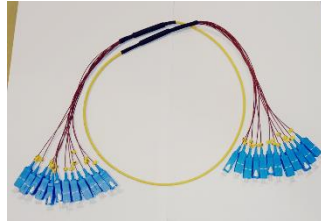
3mm Cable with 12F 0.9mm SC/PC Breakout
